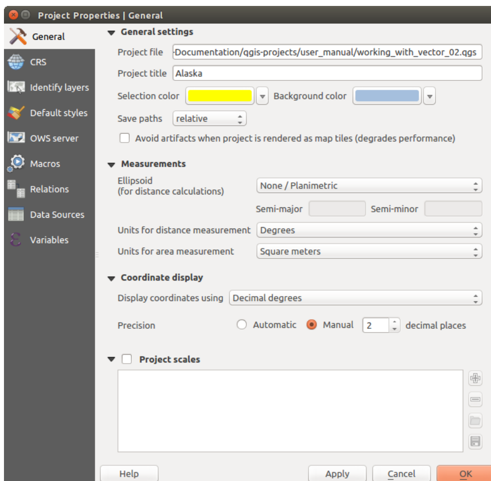
Figure 9.4: General tab of Project Properties dialog
