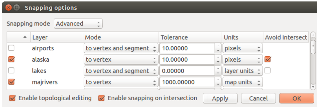
Figure 12.69: Edit snapping options on a layer basis (Advanced mode)
